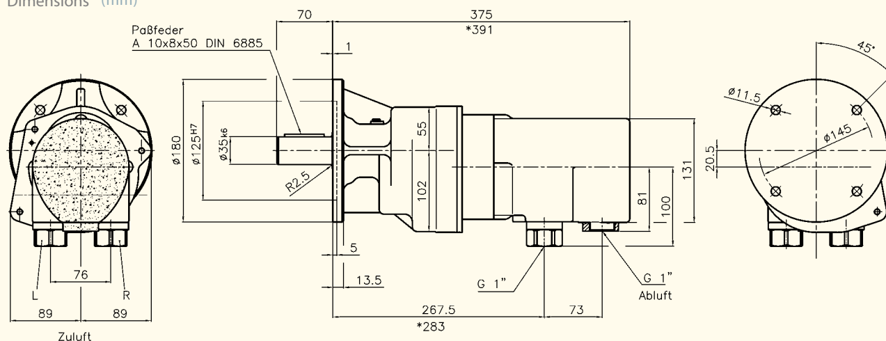
Dimensions (mm)
