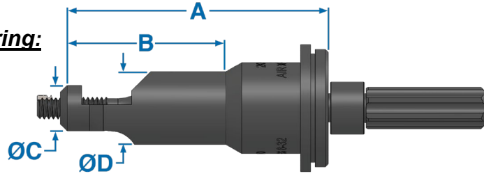
CT5420-PA Adapter for KFS-12
